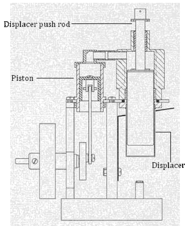
Fig(32): A cut section drawing of a Ringbom engine.
