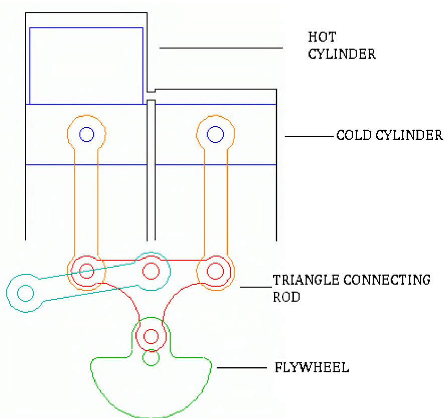
Fig(14): An Alpha Stirling engine with a Ross Yoke drive*.
