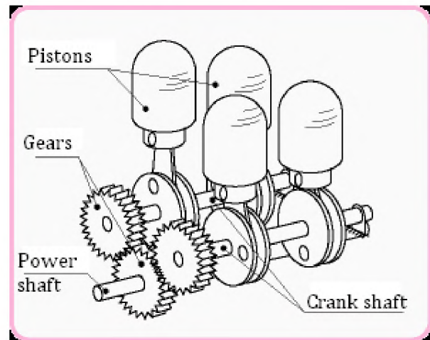
Fig(17):Gear mechanism
