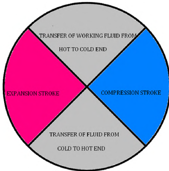
Fig(22): Position of piston on flywheel for different strokes for a vertical Beta engine.
