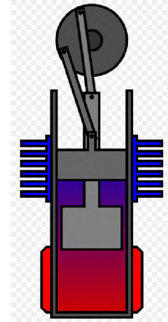
Fig(22): Position of piston on flywheel for different strokes for a vertical Beta engine.
