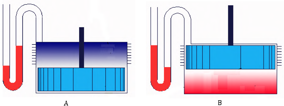
Fig(36): A fluidyne engine with solid displacer and liquid piston. Figures A and B indicate two different strokes.
